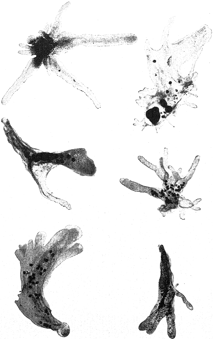
Idiochromidia formation in Amoeba proteus . (After Calkins.)
